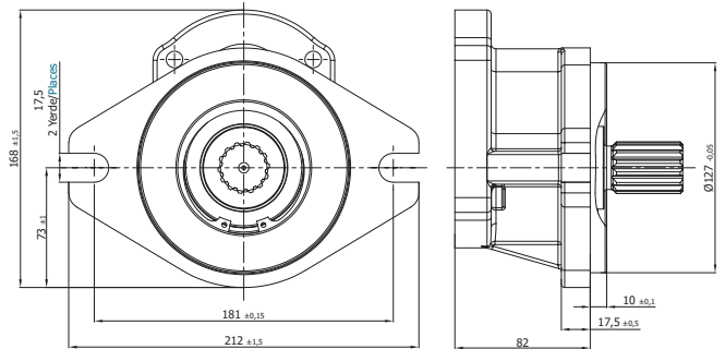
SAE 'C' 2 BOLTS P
