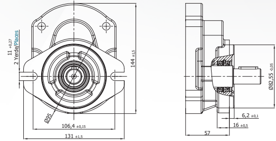
SAE 'A' 2 BOLTS B
