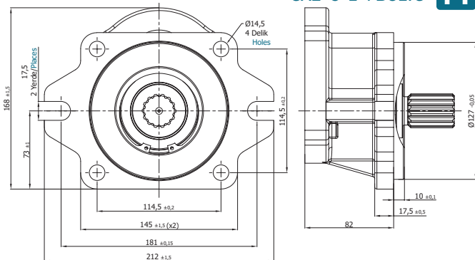
SAE 'C' 2-4 BOLTS P1
